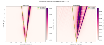
Figure: Supershear and Sub-Rayleigh F-k spectra with medium and Lamb-wave dispersion curves indicated by colored lines.
